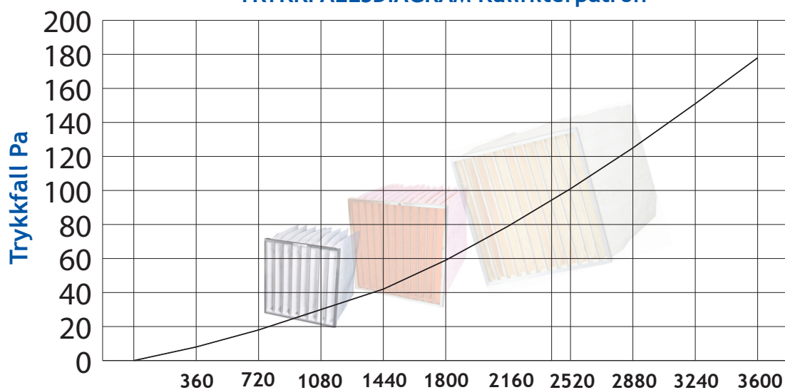
TRYKKFALLSDIAGRAM Kullfilterpatron
