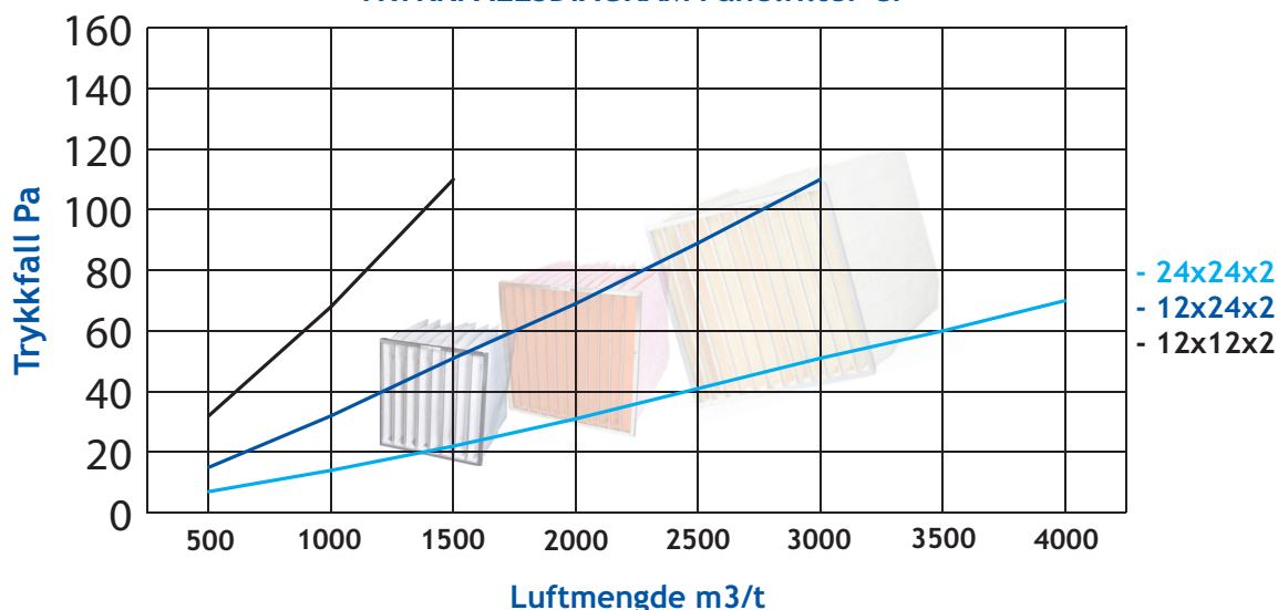
TRYKKFALLSDIAGRAM Panelfilter CP
